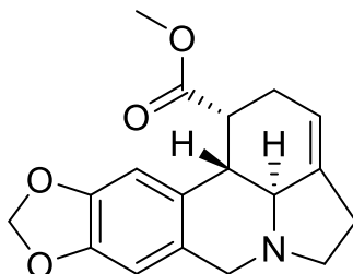
Fig. 1. The identified structure of acetylcaranine 1
