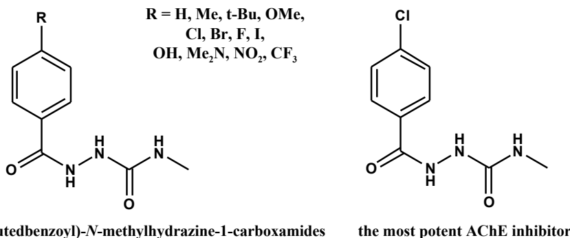
Fig. 1 Structures of the studied compounds
