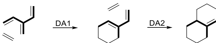
Scheme 2. Diels-Alder reactions
