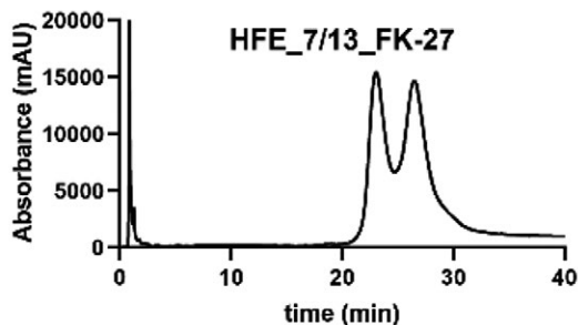
Fig. 1. Chromatogram of probe modified by FK-27
