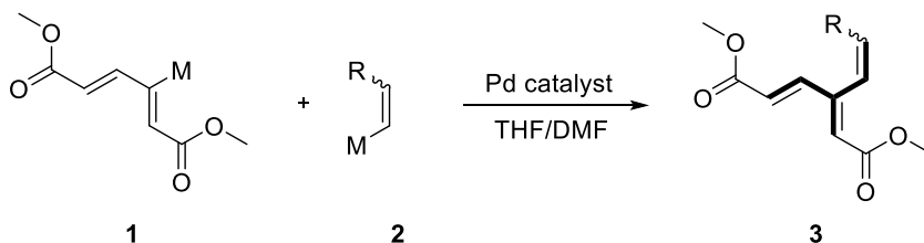
Scheme 1. Migita-Stille coupling
