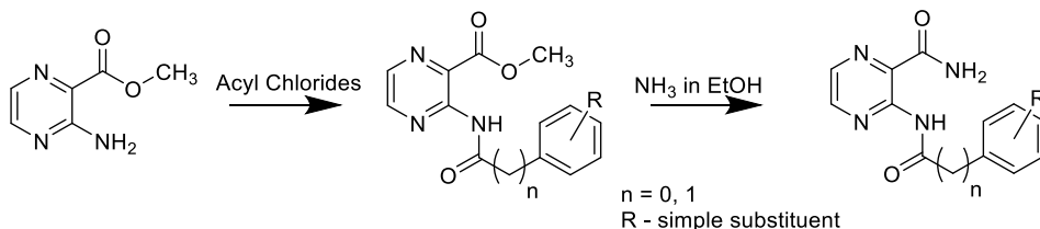
Scheme 1. Synthesis of final compounds
