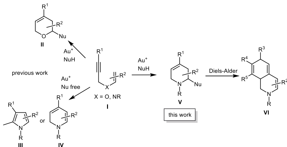
Scheme 1. Gold(I)-Catalyzed Synthesis of Piperidine Aminals
