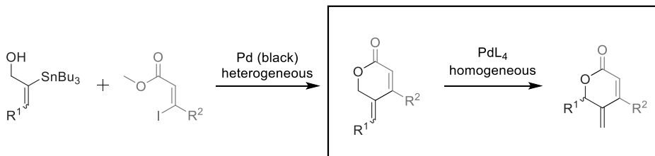
Scheme 1. General structures
