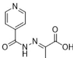
Fig. 1. (E)-2-(2-Isonicotinoylhydrazinylidene)propanoic acid
